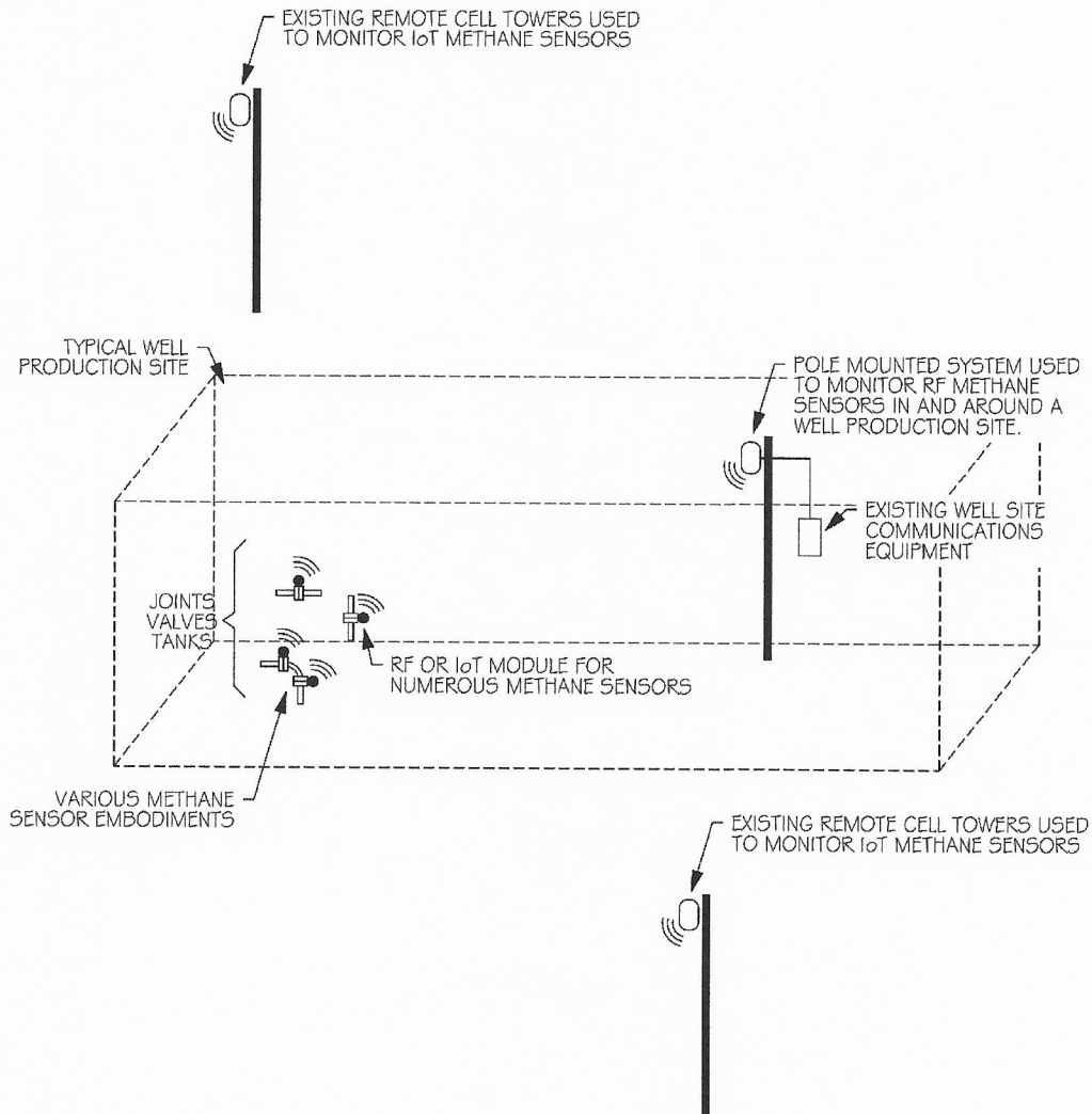
Figure 1: Topology of the proposed methane sensor communications.
