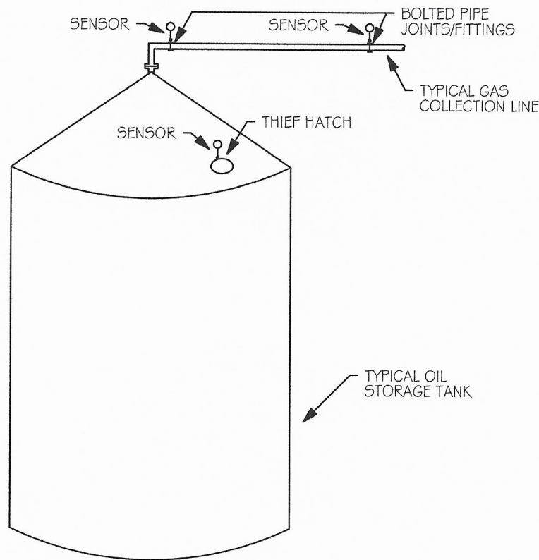
Figure 1: Typical Well Site Storage Tank
