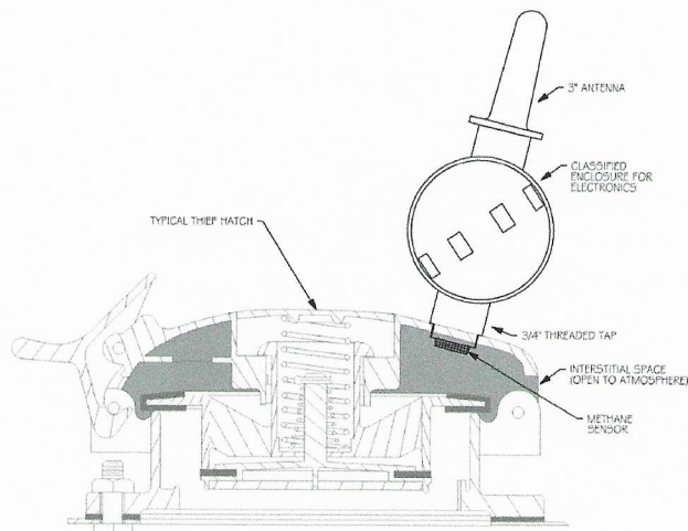
Figure 2: Typical Thief Hatch with Sensor Attached
